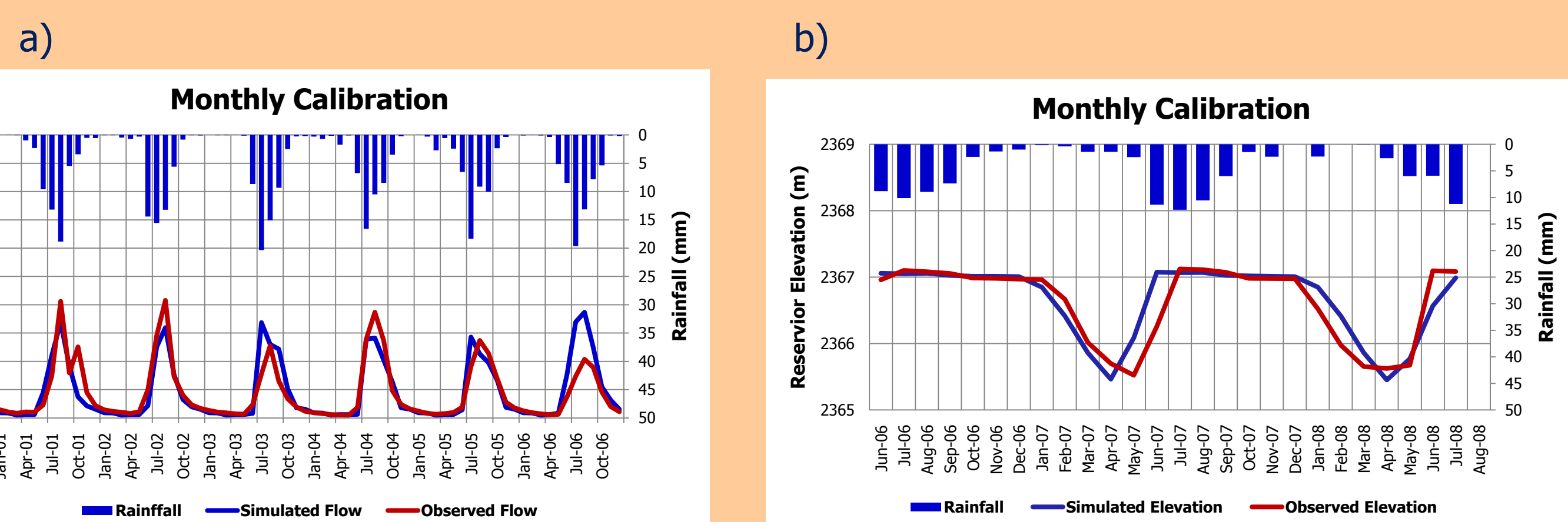
Figure 1: Calibration results for a) Koga and b) Gomit Reservoirs
