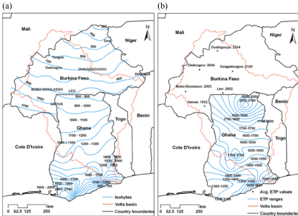
FIGURE 8. (a) Rainfall; and (b) Potential evaporation in Ghana (Source: Barry et al. 2005).
