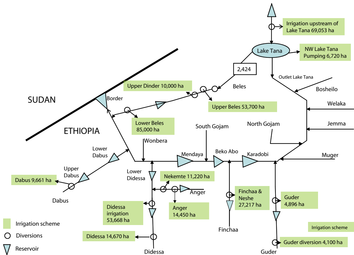
FIGURE 5. Schematic of proposed large-scale storage and irrigation schemes in the Abay Basin that could be implemented over the next 20-40 years (Source: adapted from McCartney et al. 2009).
